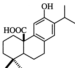
Pisiferic acid
